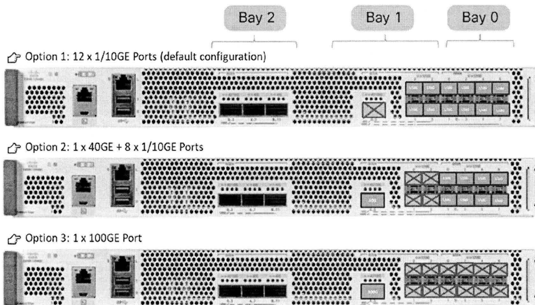
Figure 5. Bay 0 + bay 1 port options
