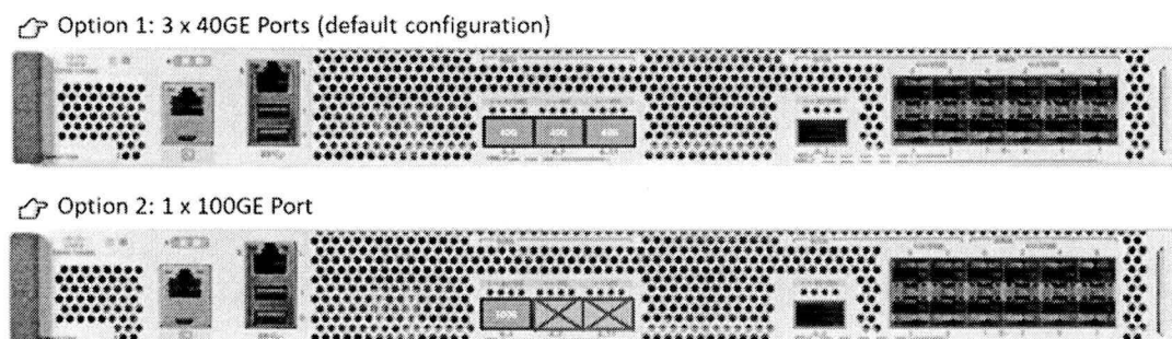
Figure 6. Bay 2 port options
