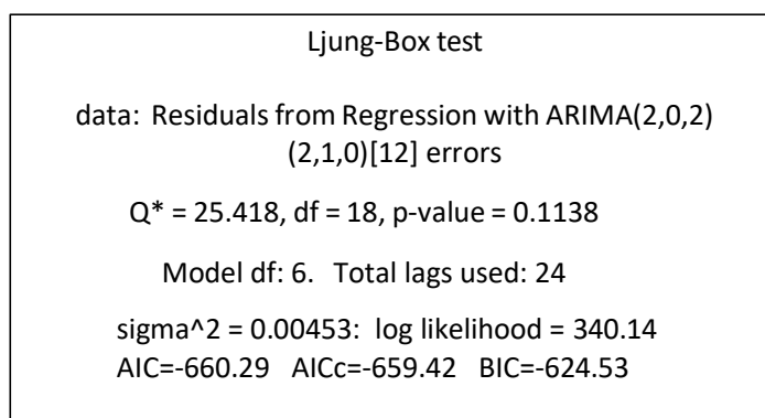
Figura 3: Teste Ljung-Box
